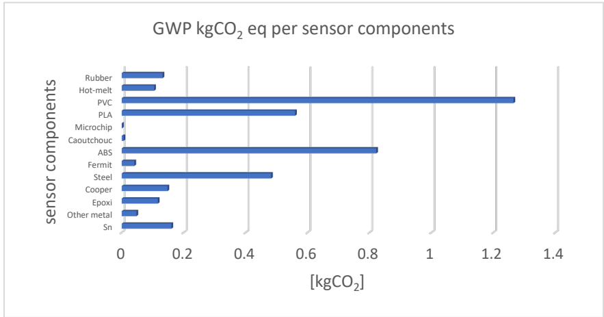
Figure 6 GWP per sensor component
