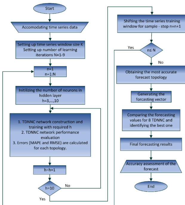
Figure 3 Extended short term neural prediction algorithm
