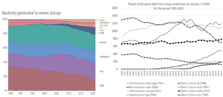
Figure 1 a) European electrical energy production profile over years [42], and b) Illustration of European electrical energy production time series by sources
