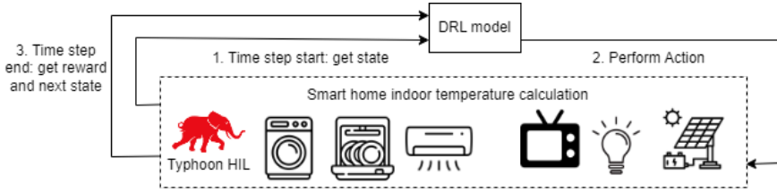
The architecture of the environment. The DRL model is either PPO or DDQN.
