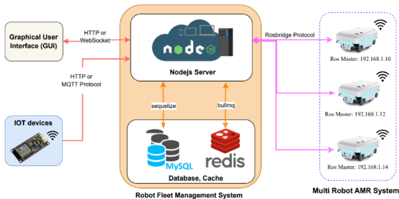
Figure 4 Communication Diagram in FMS System
