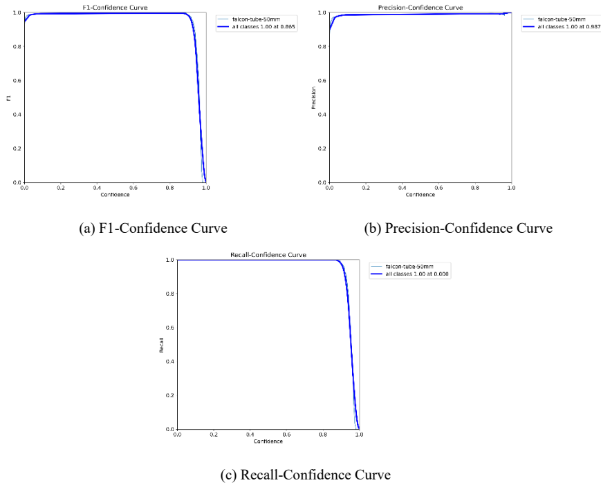
Figure 13 Confidence curves of YOLOv8 after training
