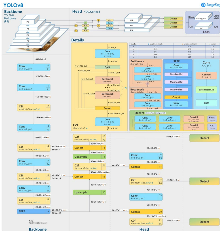
Figure 3 YOLOv8 Architecture
