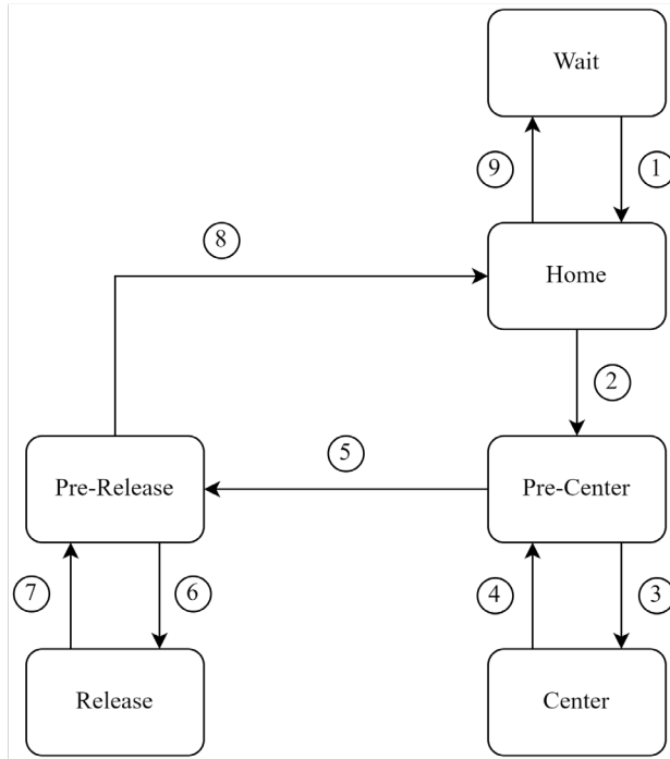
Figure 12 Pick-and-place sequence for each tube diagram
