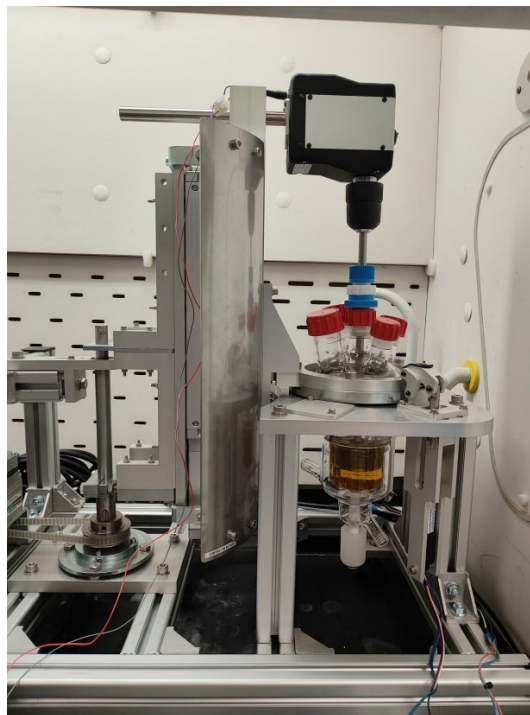
Figure 5 Experimental Testing of the Automated RBR
