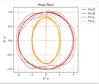
Figure 7 Phase trajectory tracking of the adaptive SMC controller with Steffensen, and without noise
