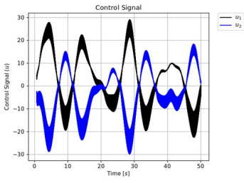
Figure 6 Control force of the Adaptive SMC controller without Steffensen , and noise
