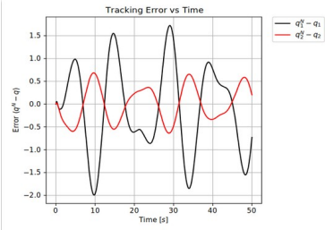
Figure 5 Trajectory tracking error of the adaptive SMC controller without Steffensen, and simulated noise
