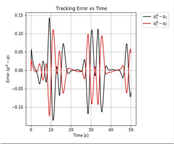
Figure 8 Trajectory tracking error of the Adaptive SMC controller with Steffensen , and without noise
