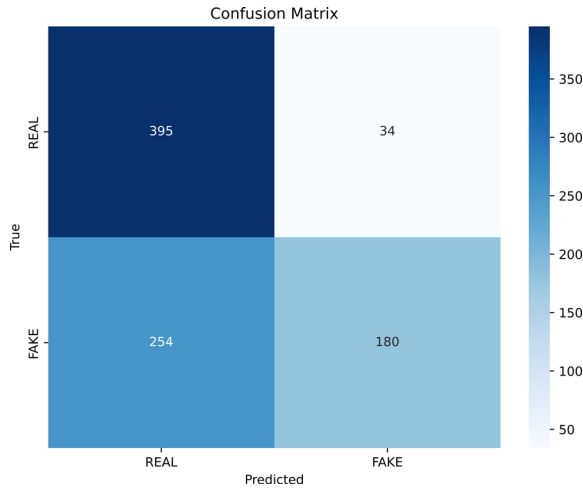
Figure 4 Confusion Matrix
