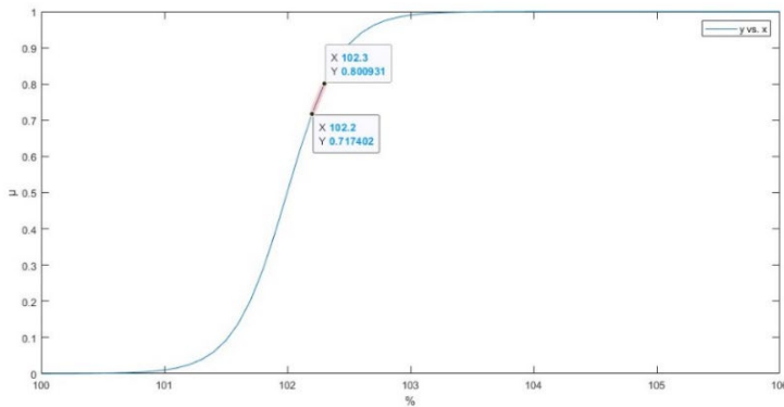
Figure 5 Sigmoid function
