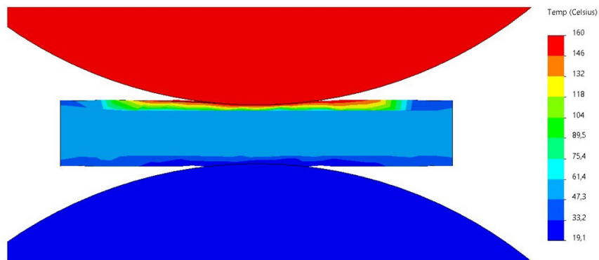
Figure 4 Distribution of the temperature inside the rollers and the copper core cable (outer diameter of the cable – 6.8 mm)
