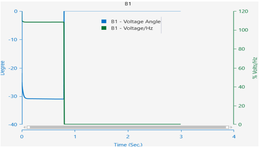
Figure 7 Bus 1, behavior parameters at the time of the fault at the equivalent 100 kV level grid
