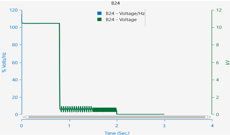
Figure 6 Bus 24, behavioral parameters during faults (connected PV and WT)
