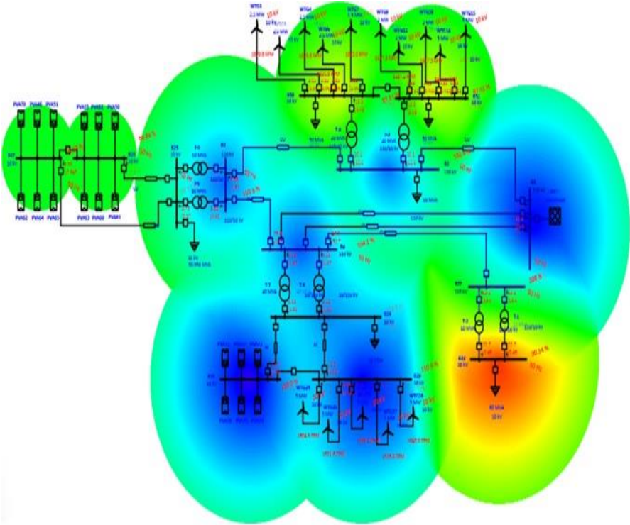
Figure 2 Integration of wind turbines and PV systems (case study)
