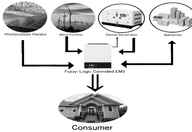
Figure 2 Structure of a OMPGS system
