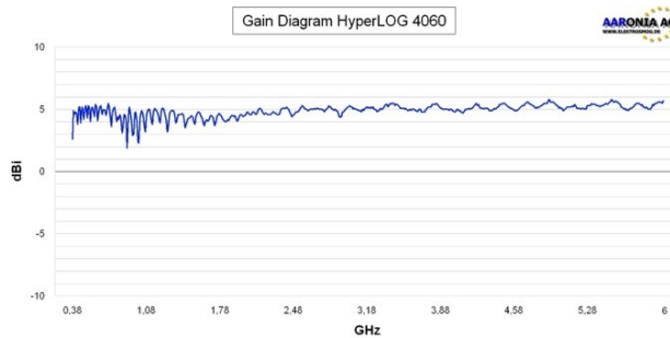
Figure 4 Antenna gain in dBi of HyperLOG broadband antenna [11]
