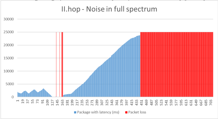
Figure 20 II.hop - Noise in full spectrum
