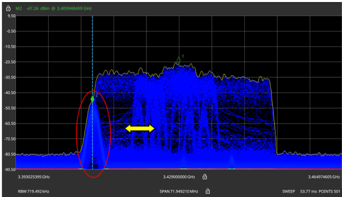
Figure 15 Snapshot of the sweep jamming
