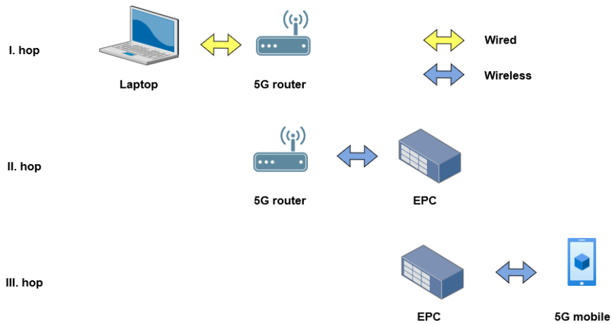
Figure 2 Packet transfer topology
