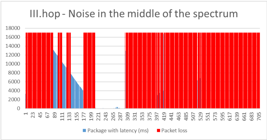
Figure 11 III.hop - Noise in the middle of the spectrum
