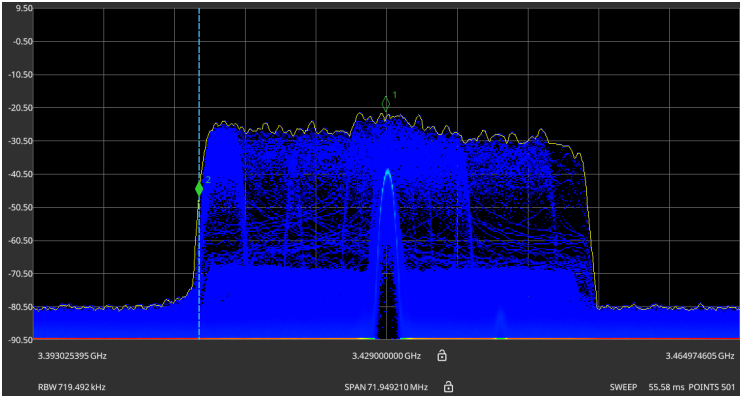
Figure 9 Spectrum during the jamming (middle of the band)
