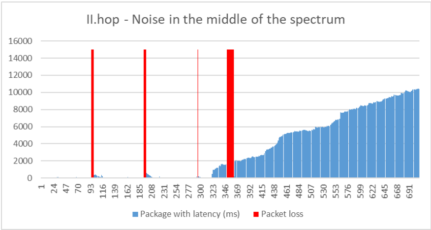
Figure 10 II.hop - Noise in the middle of the spectrum
