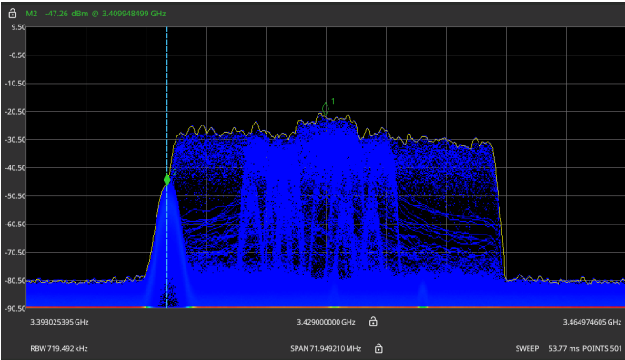
Figure 7 Spectrum during the jamming (start of the band)
