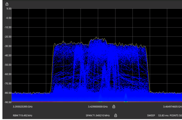
Figure 3 Reference radio spectrum
