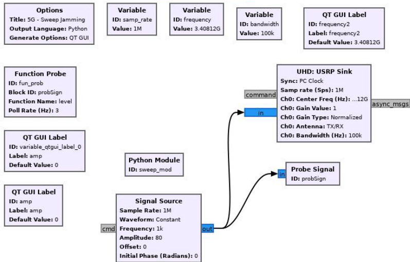
Figure 14 Sweep jamming method
