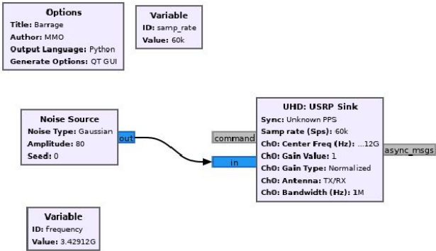
Figure 8 Jamming at 3.42912 GHz (middle of the band)
