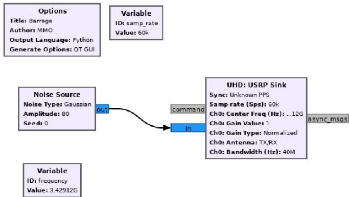
Figure 18 III.hop – Sweep noise
