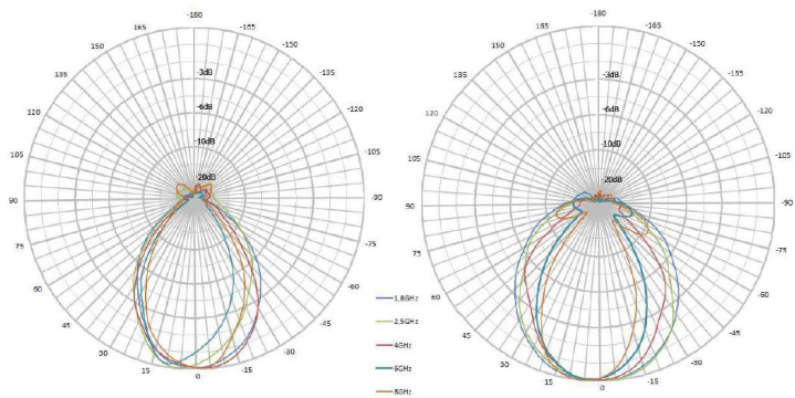
Figure 5 Antenna horizontal and vertical radiation pattern plots of HyperLOG 4060[6]
