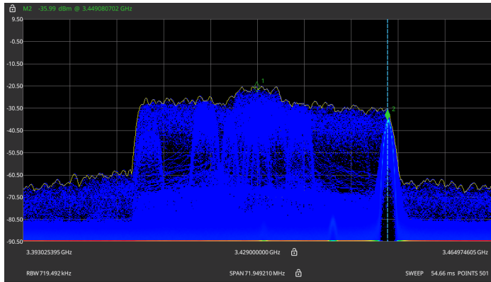
Figure 13 Spectrum during jamming (end of the band)
