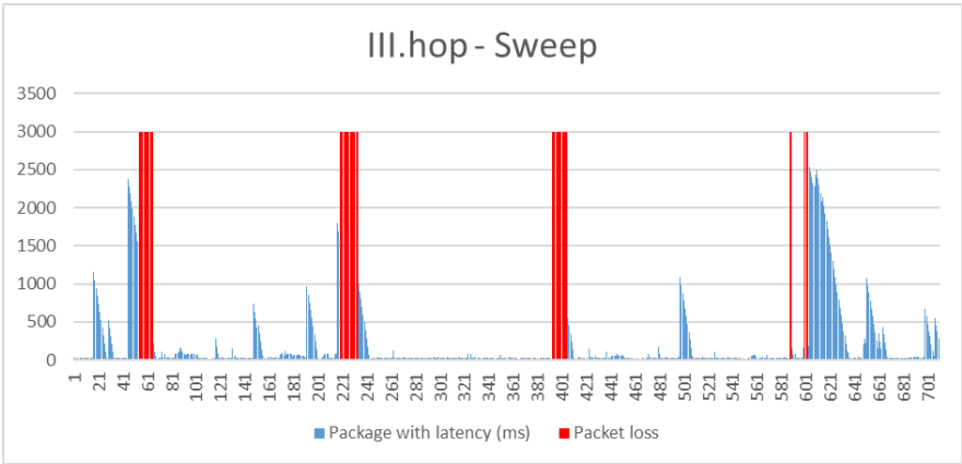
Figure 17 III.hop – Sweep noise
