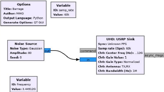
Figure 12 Jamming at 3.44912 GHz (end of band)
