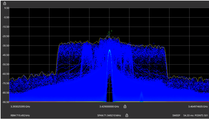
Figure 19 Spectrum of the jamming in the whole 5G SA band
