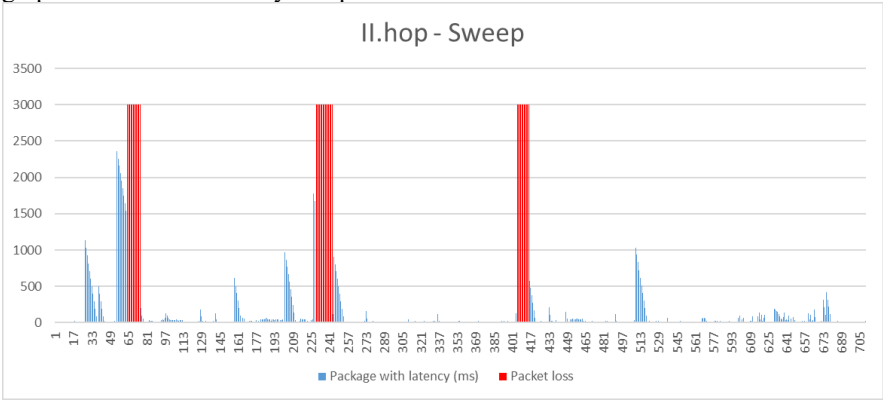
Figure 16 II.hop – Sweep noise
