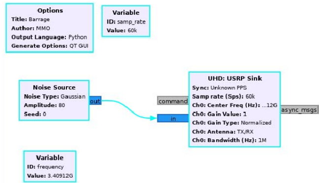
Figure 6 Jamming at 3.40912 GHz (start of the band)
