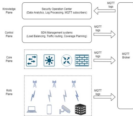
Figure 5 Implementation of SDN and MQTT [34]
