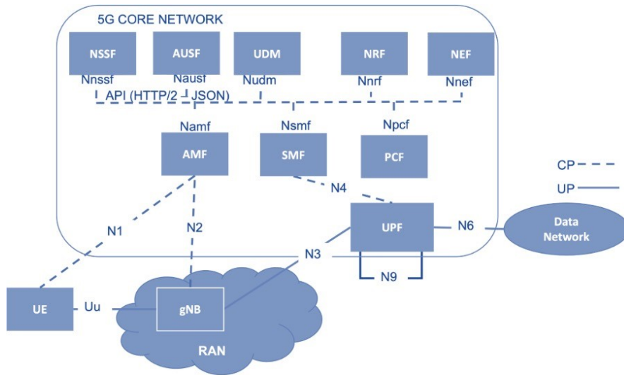
Figure 1 The architecture of 5G network
