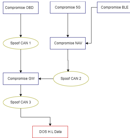
Figure 6 Attack graph for a DOS attack
