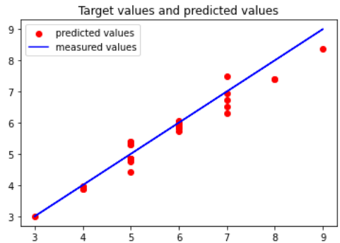
Figure 2 Original target values vs. predicted values
