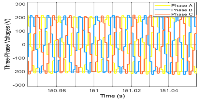
Figure 12 Advanced Powertrain Three-Phase Voltages
