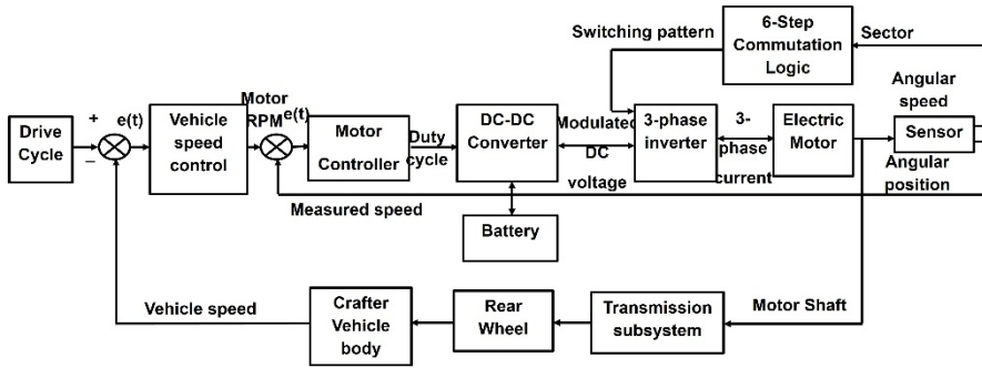
Figure 4 Advanced Powertrain Model [11]
