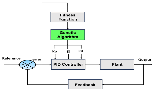
Figure 8 GA-PID Structure [29]
