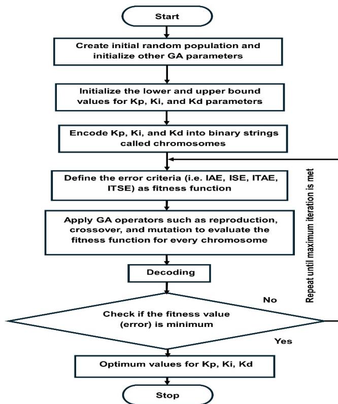
Figure 9 GA Flowchart [29]
