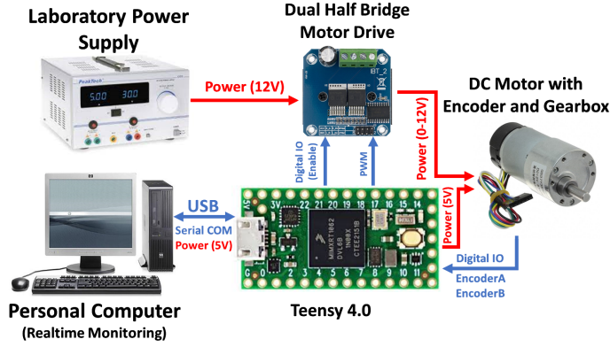
Figure 5 Simple Block Diagram of the Experimental Setup
