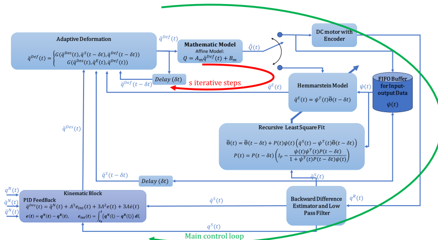
Figure 3 Improved RFPT control with model identification and multiple adaptive steps
