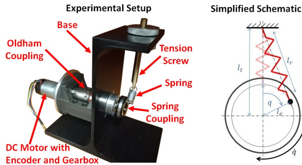
Figure 4 Mechanical design of the experimental setup (left) and simplified dynamic model (right)
