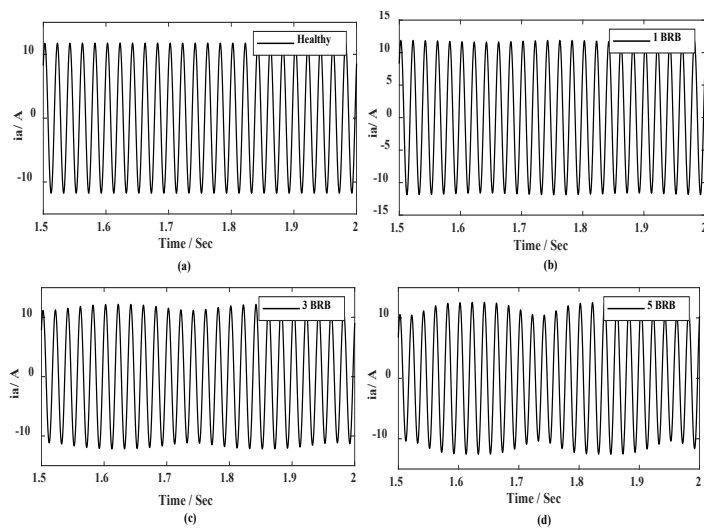
Figure 2 Stator current for (a) healthy condition, (b) one broken rotor bar, (c) three broken rotor bars, and (d) five broken rotor bars
