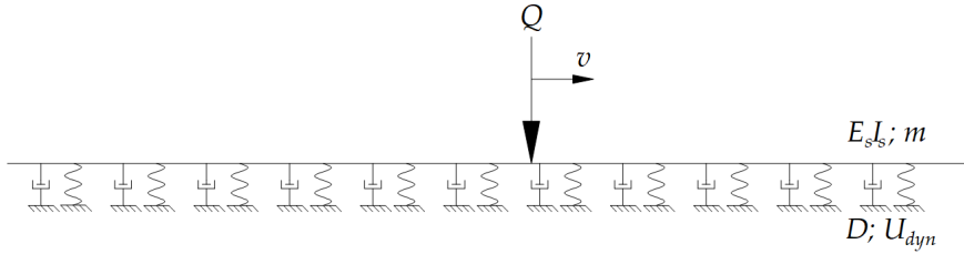
Figure 1 The model of the dynamically loaded structure
