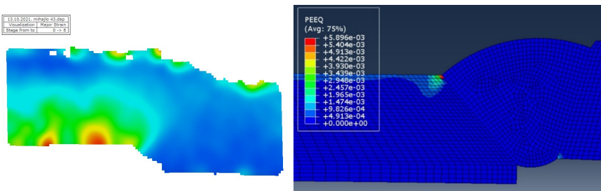
4 th group specimen - strain field: left) obtained by DIC; right) FEA
