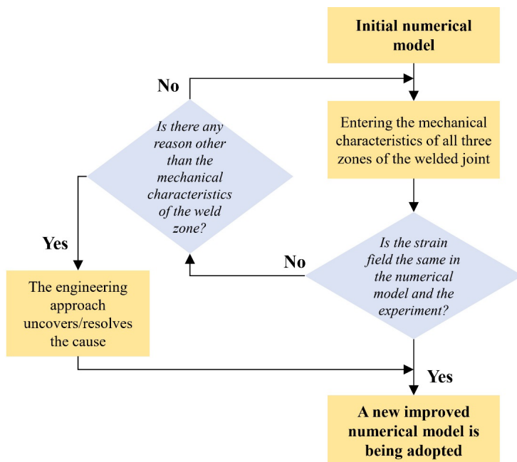
Figure 2 Algorithm of inverse iterative methodology (IIM)
