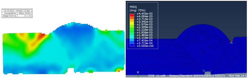
1 st group specimen - strain field: left) obtained by DIC; right) FEA
