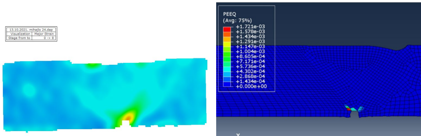
2 nd group specimen - strain field: left) obtained by DIC; right) FEA
