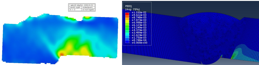
3 rd group specimen - strain field: left) obtained by DIC; right) FEA
