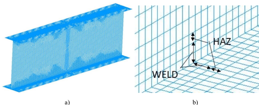
Figure 5 FE model of I profile shape girder, a) plate elements; b) zone dimensions
