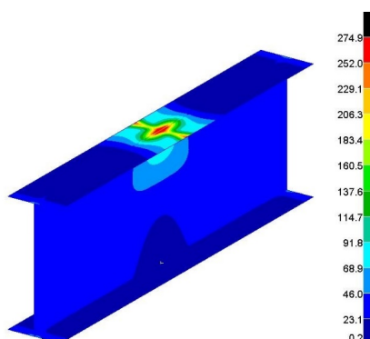
Figure 11 Von Mises stress [MPa] for linear elastic analysis of the girder containing welded joints loaded with F = 147\,060\text{ N}
