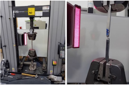
Figure 15 Instron 5582 universal tensile testing machine during the tensile tests
