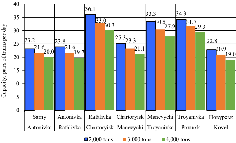
Figure 2 Capacity per section on the Kovel-Sarny route
