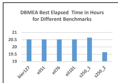
Figure 5 Best elapsed time in hours for different benchmarks with DBMEA
