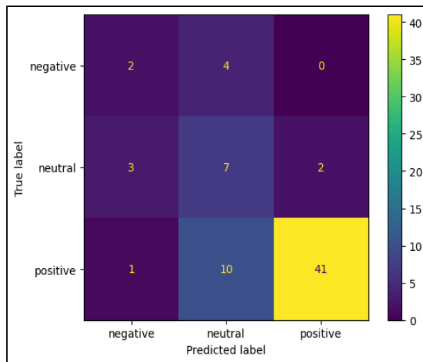
Figure 3 Confusion matrix
