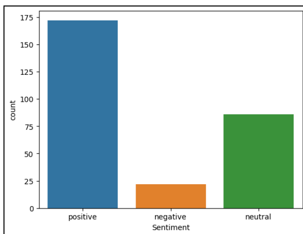
Figure 2 Classification result
