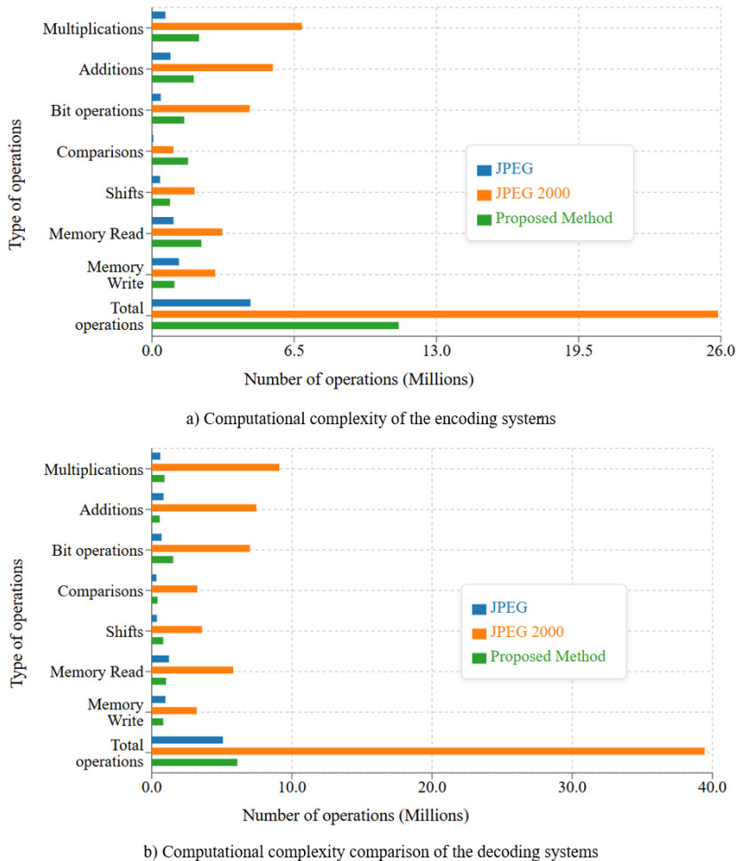
Figure 12 Computational complexity of the three implemented systems
