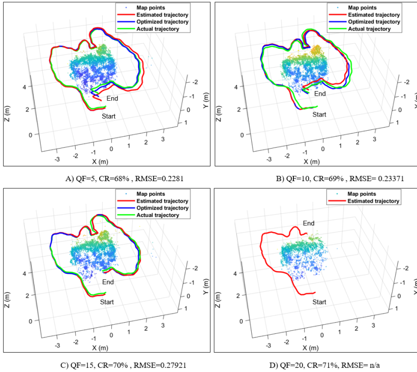
Figure 8 ORB-SLAM trajectory estimation performance adopting JPEG compression
