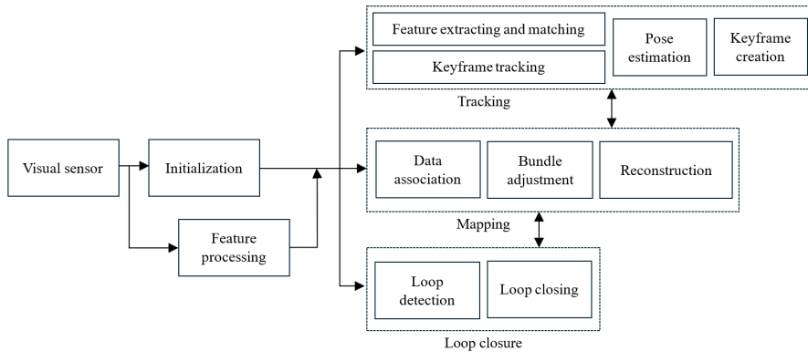
Figure 1 ORB-SLAM Architecture
