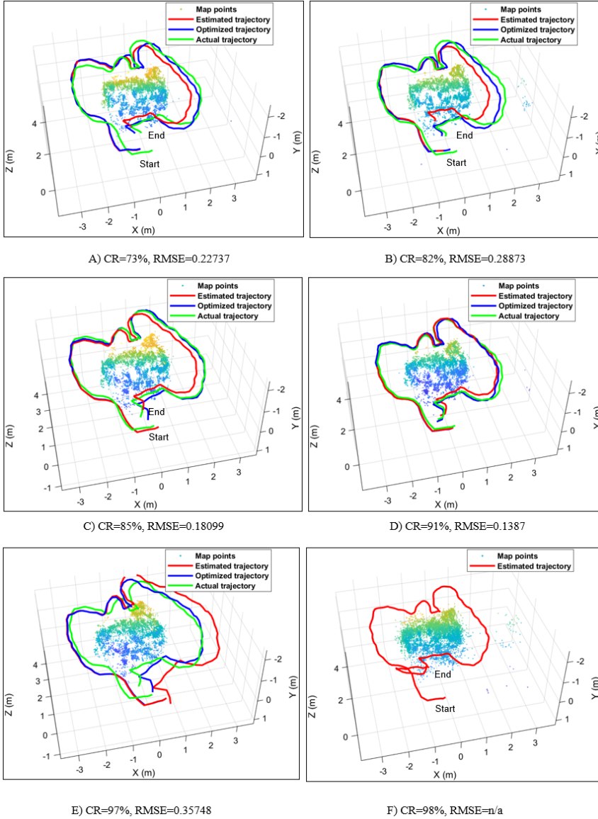
Figure 9 Trajectory estimation performance of ORB-SLAM system adopting JPEG 2000
