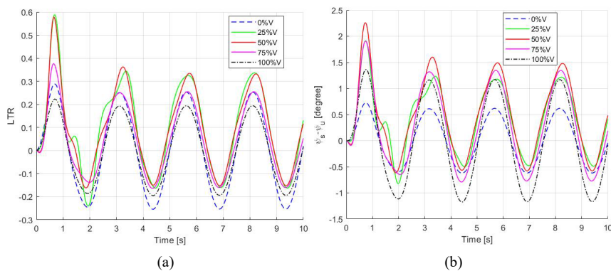
Figure 4 The LTR (a) and RAS (b) value in lane change
