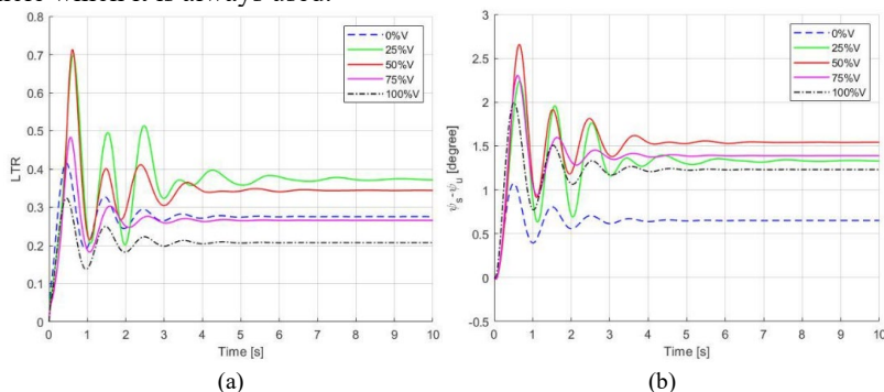
Figure 3 The LTR (a) and RAS (b) value in steady turning
