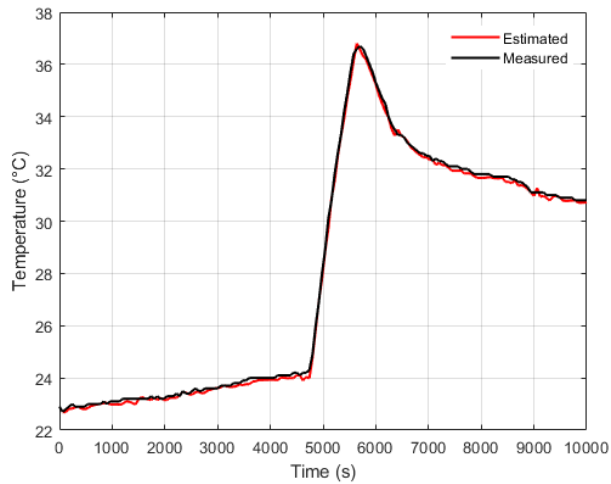
Figure 10 Comparison of measured and estimated temperature
