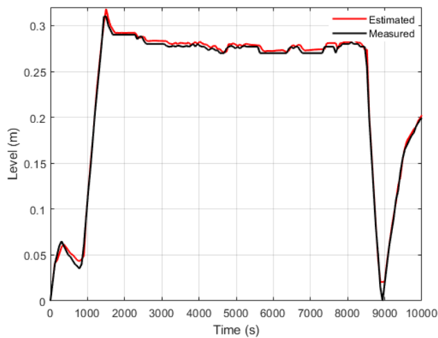
Figure 11 Comparison of measured and estimated level
