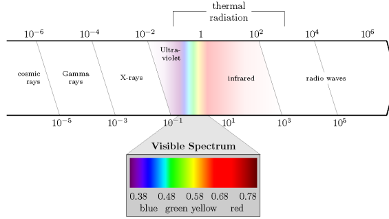
Figure 1 Electromagnetic Spectrum
