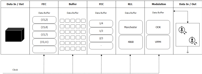
Figure 3 Block structure
