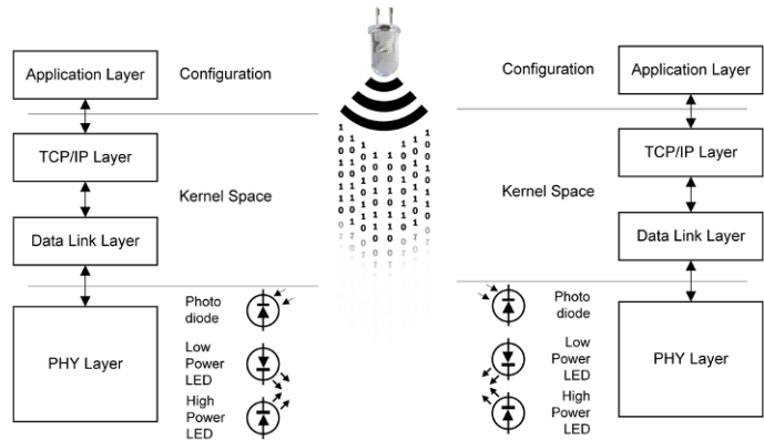
Figure 2 Block structure
