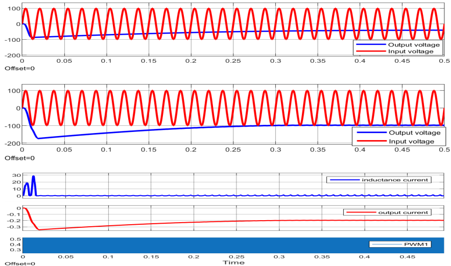
Figure 15 Output voltage at D=30 and D=60 for the conventional converter with currents and PWM
