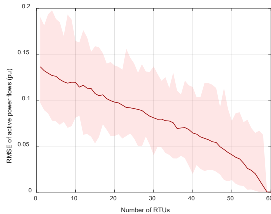
Figure 6 Impact of RTUs penetration on estimated power flows
