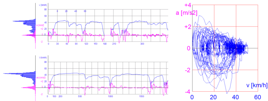
Figure 9. Speed and acceleration representations (urban conditions): left – histograms; middle – fragments from plots vs. time (up) and vs. distance (down); right – city driving cycles
