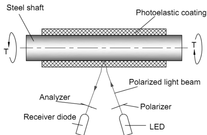
Figure 2. Test equipment
