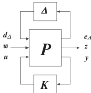
Figure 3: The P - K - \Delta structure
