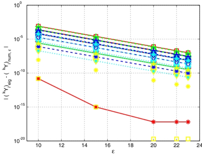
Figure 1. Difference of the numerically integrated values {}^kY_\ell from their counterparts calculated with an eigenvalue equation of matrix M_{k,\ell}^{[0]} as a function of the grid points in a unit interval 2^\epsilon . Red color with continuous line means k = 0 , green with dash-dot line mean k = 1 , blue with dashed line k = 2 , cyan with dotted line k = 3 and the color yellow and markers without line means k = 4 . The markers * , \nabla , \circ , + , and \square stand for the indices \ell = k - 4 , k - 3 , k - 2 , k - 2 and k respectively.
