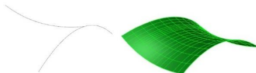
Figure 3. Constructing the saddle-surface [9]
