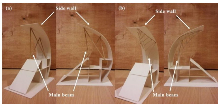
Figure 9. Variations for the main beams
