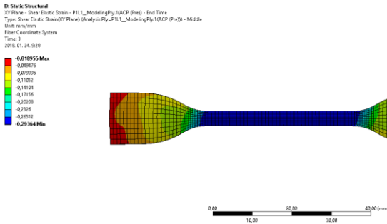
Figure 10. Strain in plane 12, ply1
