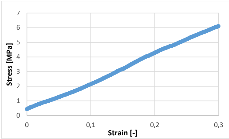
Figure 3. Stress-strain curve of rubber test specimen at -40 °C
