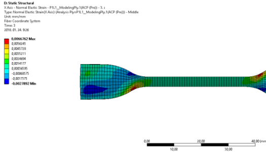
Figure 9. Strain in material direction 1, ply1
