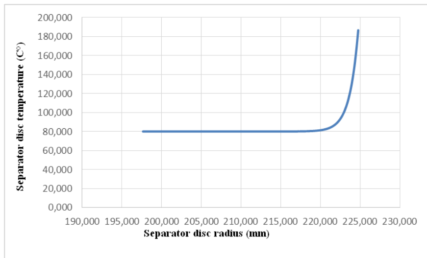
Figure 5. Radial heat change of the separator disc
