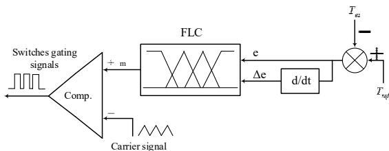
Figure 4. PD-Fuzzy logic direct torque control
