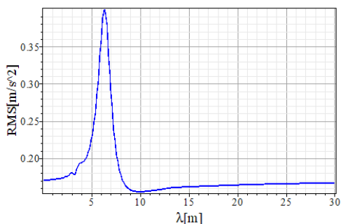
Figure 8. Sensitivity of wavelength of the road
