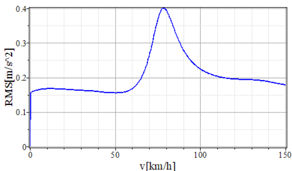
Figure 6. Sensitivity of the vehicle speed
