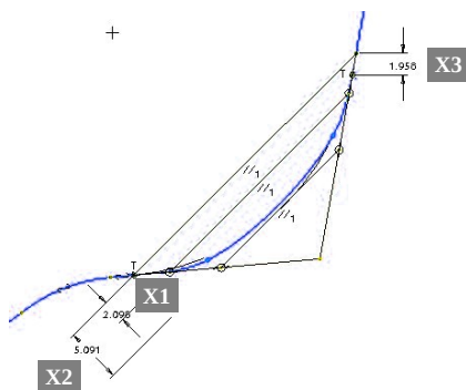
Figure 6. The variable dimensions of the spline4.3 curve
