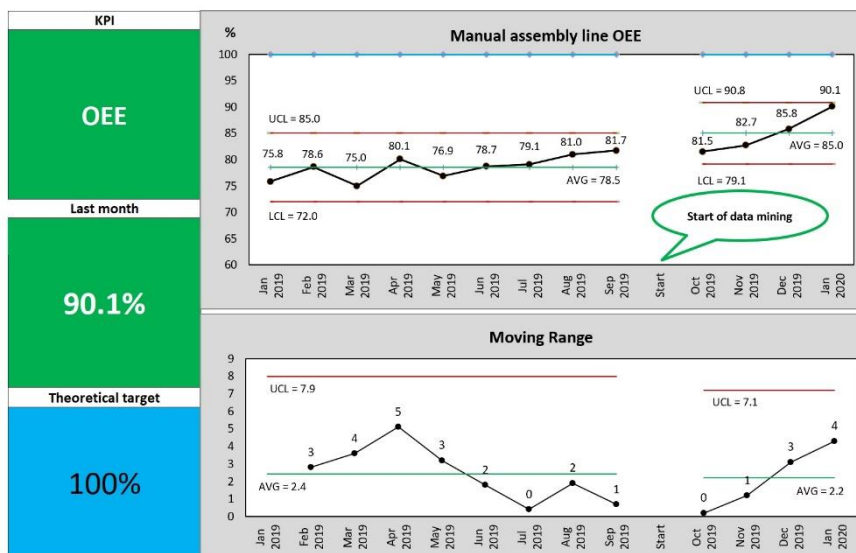
Figure 9. OEE improvement
