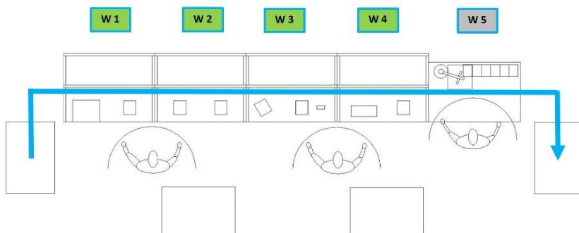
Figure 5. Manual assembly line
