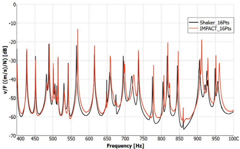
Figure 9. RMS average of 16 response points for shaker and impact excitation cases. The excitation point and the response points were at the same locations for both cases.
