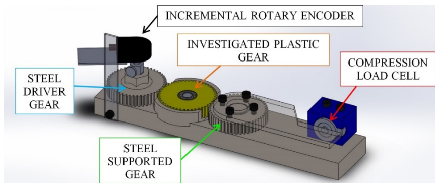
Figure 1. Test rig for overload test
