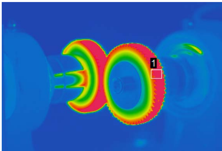
Figure 8. Thermal image of PA6 gears with sampling area
