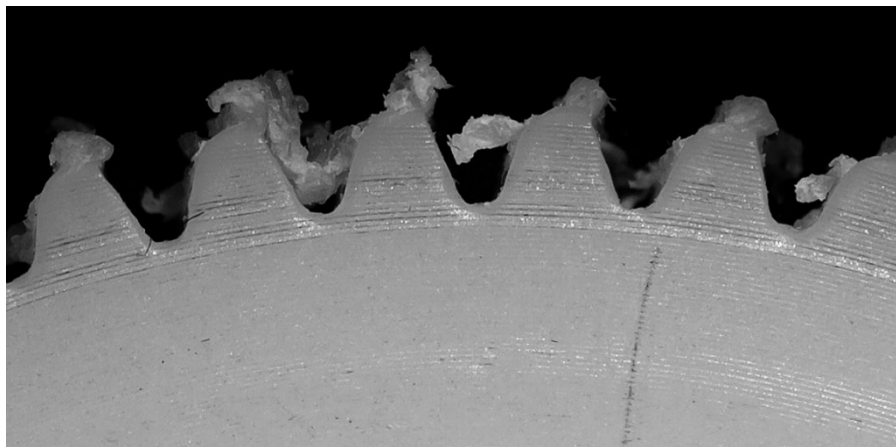
Figure 10. The melting of the teeth of a PA6 gear
