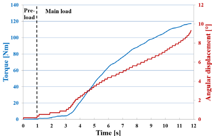
Figure 4. An overloaded test of PA6 gear with lower stress rate
