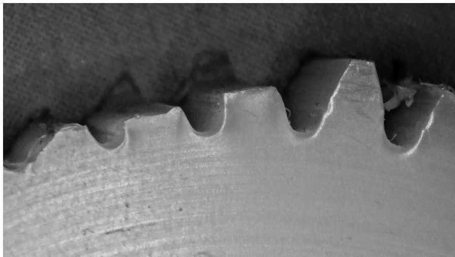
Figure 7. The fractured teeth of a POM gear
