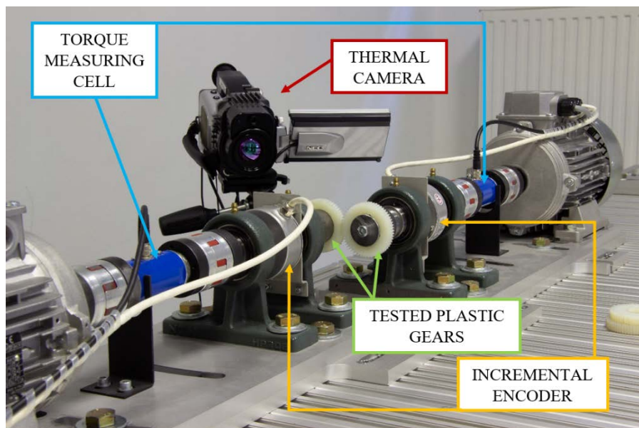
Figure 2. Test rig for lifetime test
