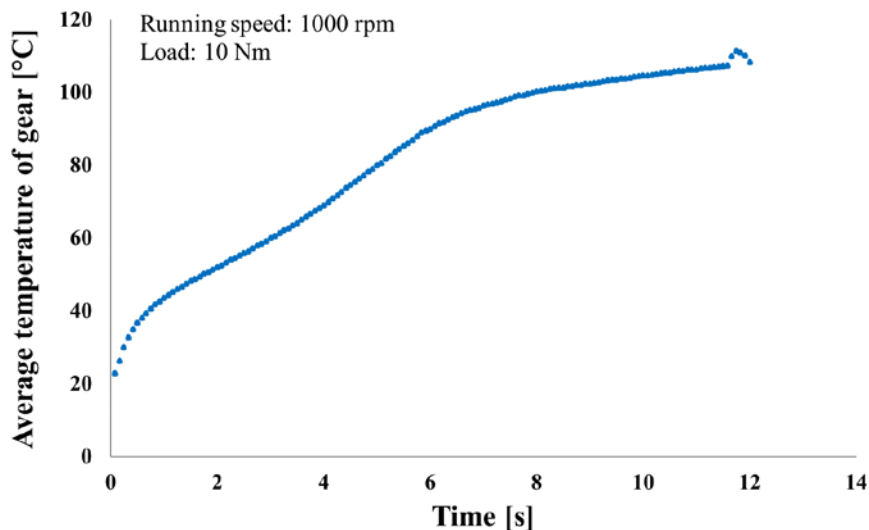
Figure 9. The heating of a PA6 gear
