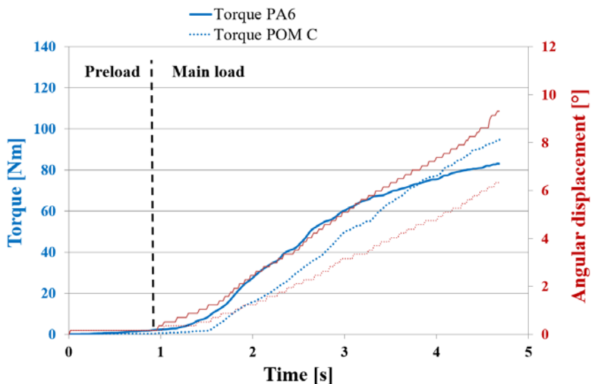
Figure 3. Characteristic curve of PA6 and POM gear in overloaded test
