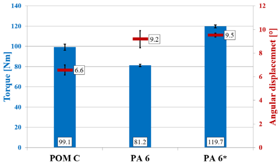
Figure 5. The main results of overloaded tests
