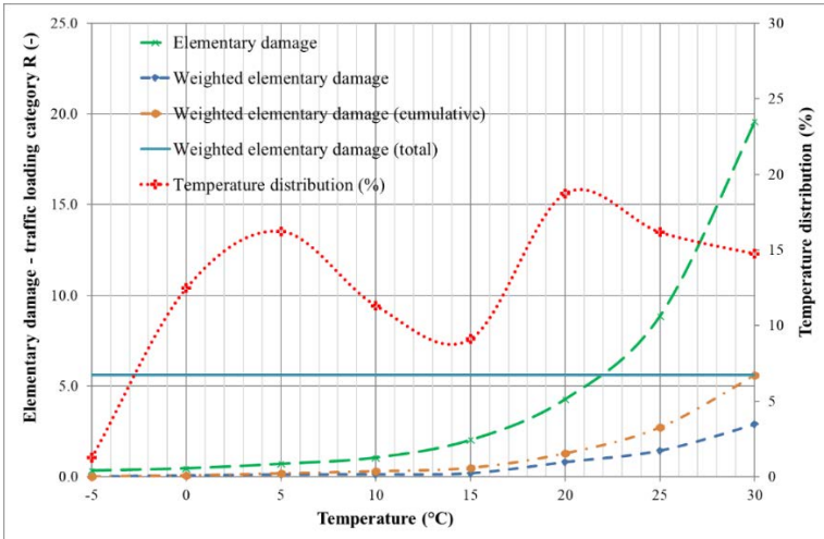
Figure 1. Establishing the equivalent temperature based on the calculation of elementary damage – traffic loading category R
