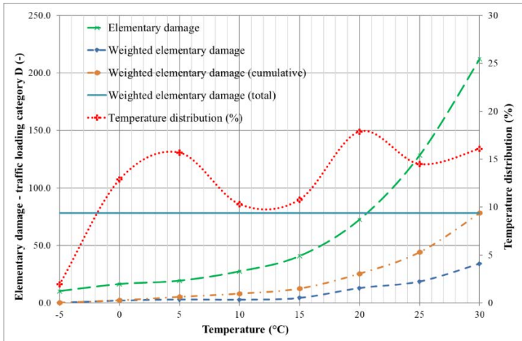
Figure 2. Establishing the equivalent temperature based on the calculation of elementary damage – traffic loading category D
