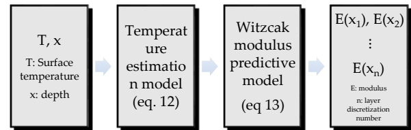
Figure 2. Scheme of modulus calculator.
