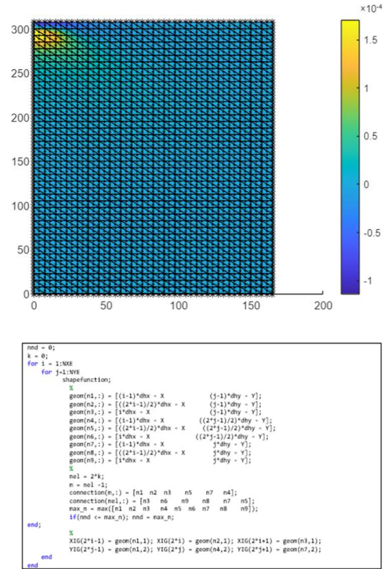
Figure 5. Mesh generation of Pave-Ut and code with horizontal strain distribution.
