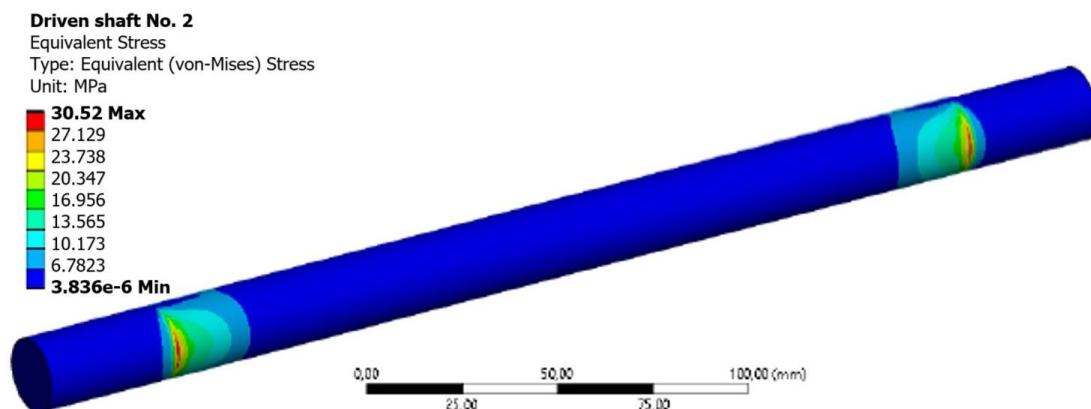
Figure 9. Reduced stress distribution in shaft No. 2
