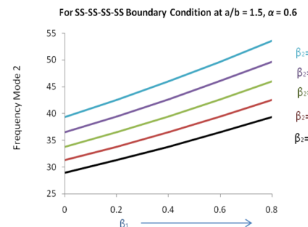
Figure 9. Frequency (Mode 2) Vs \beta_1 & \beta_2 at \alpha=0.6 , a/b=1.5 for simply supported boundary
