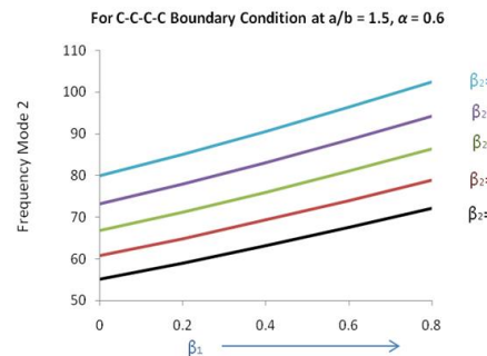
Figure 8. Frequency (Mode 2) Vs \beta_1 & \beta_2 at \alpha=0.6 , a/b=1.5 for clamped boundary
