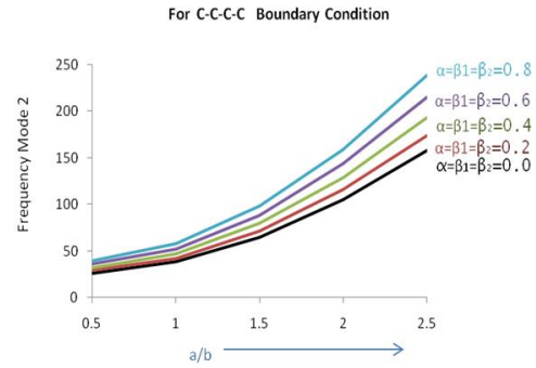
Figure 12. Frequency (Mode 2) Vs Aspect Ratio for increasing values \alpha = \beta_1 = \beta_2 for clamped boundary
