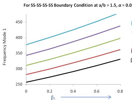
Figure 3. Frequency (Mode 1) Vs \beta_1 & \beta_2 at \alpha=0.0 , a/b=1.5 for simply supported boundary
