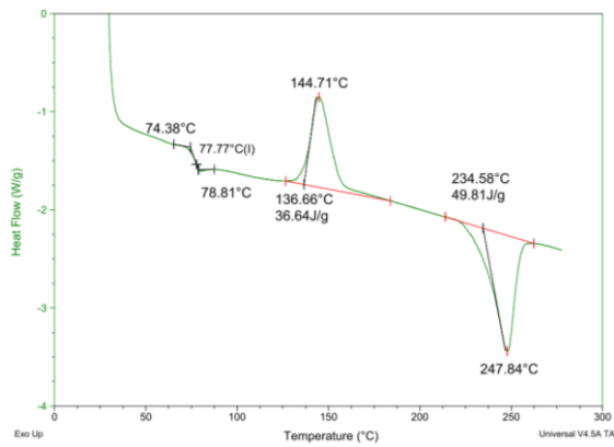
Figure 5. First heating DSC curve of an untreated PET specimen, showing the glass transition, cold crystallization, and melting peaks.
