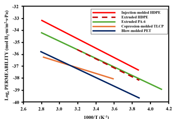
Figure 2. Temperature dependence of the hydrogen permeability for four tank liner polymers and one thermotropic liquid crystal polymer (TLCP).
